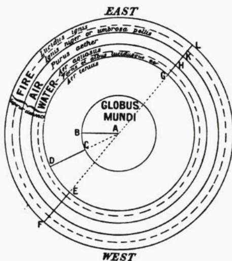
Hildegard's later scheme of the universe (reconstructed by Charles Singer).
