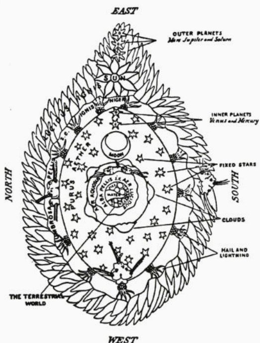
Hildegard's first scheme of the universe (simplified by Charles Singer).
